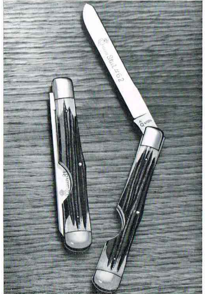
No. 62 Easy Opener Pattern — Genuine Frontier bone stag handle. Made of Queen Steel. Will not rust or stain and because of our secret tempering process, it will stay sharp far longer than other knives. Double nickel silver bolsters. Brass linings. One large spey blade, cutting edge 4 inches long. 5\frac{1}{4} inches overall when closed. Designed for skinning and castrating. Glazed finish on blades.
