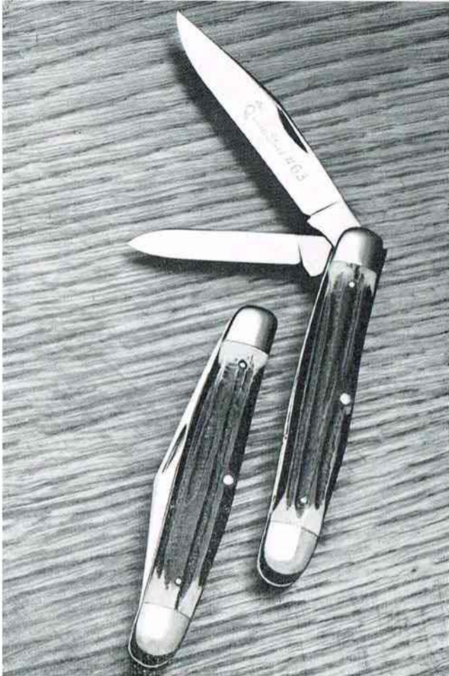
No. 63 Serpentine Pattern — Two blade jack knife. Genuine Frontier bone stag handle. Made of Queen Steel. Will not rust or stain and because of our secret tempering process, it will stay sharp far longer than other knives. Double nickel silver bolsters. Brass linings. One long clip blade 2\frac{3}{4} inches long, one pen blade 1\frac{3}{4} inches long. Overall length when closed 4 inches.
