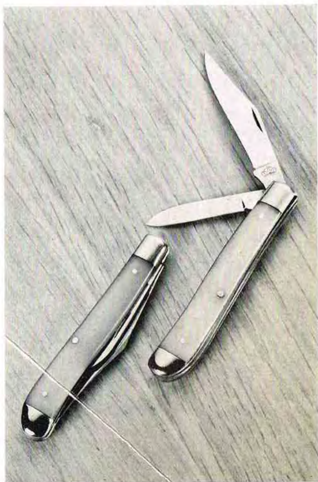
No. 17 Amber Dogleg Pattern — Two blade small jack knife. Amber handle. Double bolster, brass lined, nickel silver finish. One 2\frac{1}{8} inch clip blade and one 1\frac{7}{16} inch pen blade. 2\frac{3}{4} inches long when closed. One of our most favored patterns.
